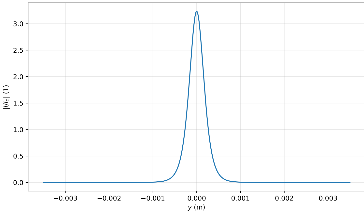
Intensity profile I(x=0, y, z=3.821)/I_0 , P_{in}=1.0P_{cr} , artificial time
